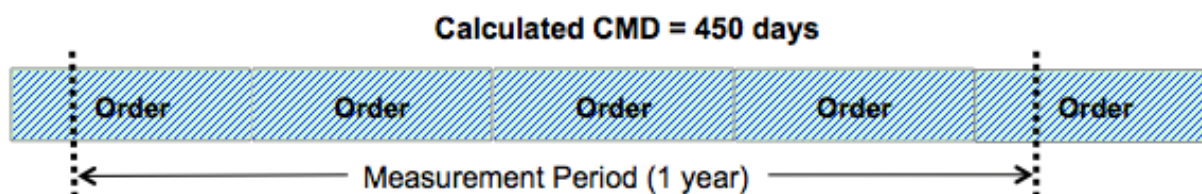
Figure 3. Cumulative Medication Duration Using Overlaps
