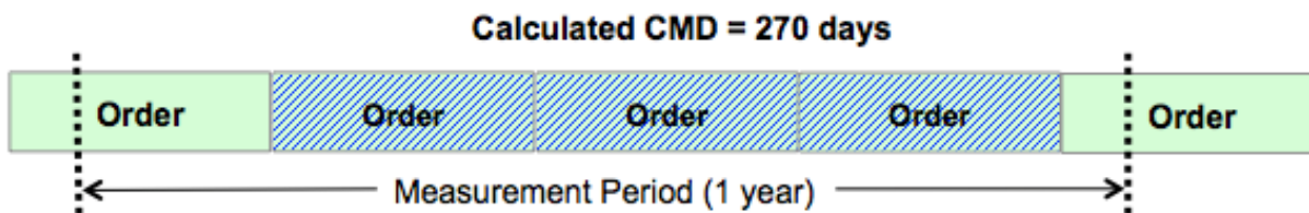
Figure 2. Cumulative Medication Duration Using During
