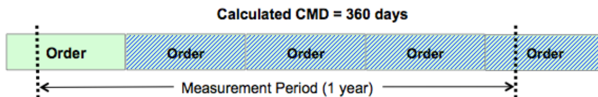
Figure 4. Cumulative Medication Duration Using Starts During
