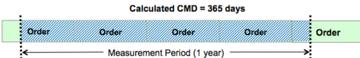
Figure 1. Ideal Cumulative Medication Duration Calculation
